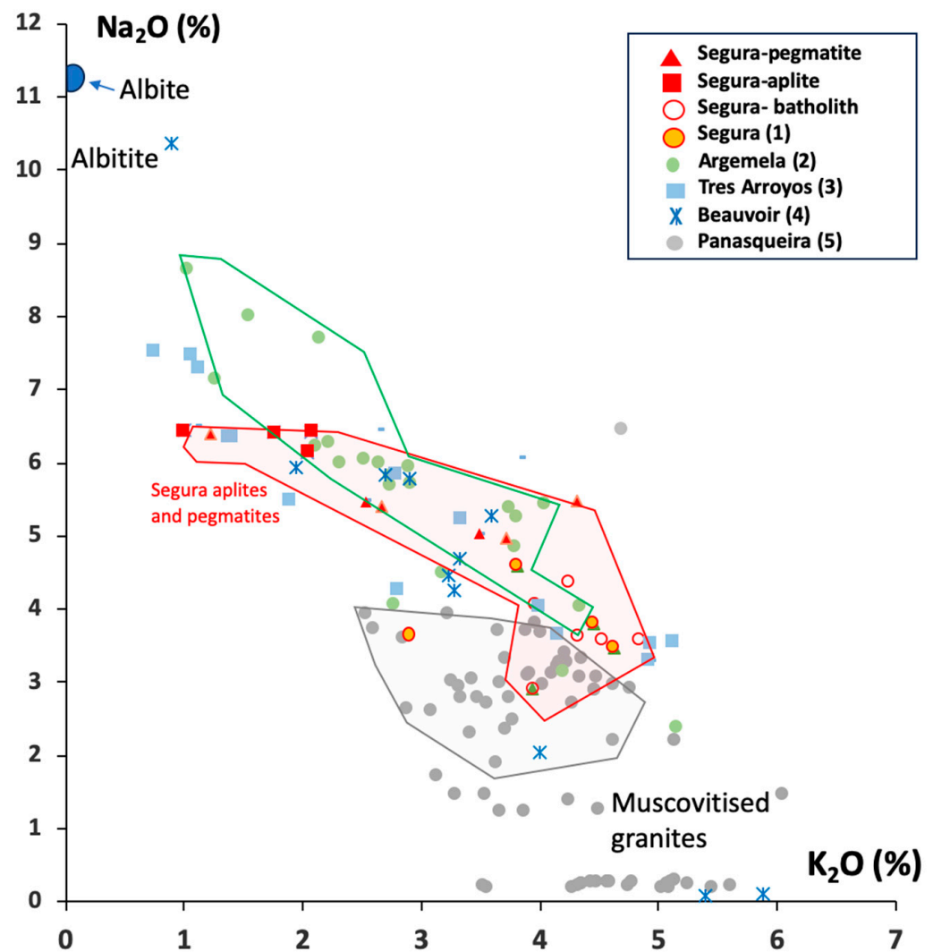
Figure 9. \text{Na}_2\text{O} versus \text{K}_2\text{O} diagram for the Segura aplites, pegmatites, and granites. Data are compared with those from the literature as follows: 1: Segura [5], 2: Argemela [10], 3: Tres Arroyos [3], 4: Beauvoir [11], and 5: Panasqueira [37]. Enveloppe colors correspond to data point colors.
